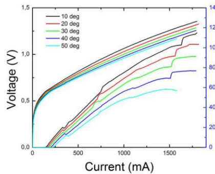
Fig. 1. Typical I - V characteristics for a 2 mm laser at different heatsink temperatures.
