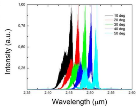
Fig. 2. Typical emission spectrum at 1300 mA at different heatsink temperatures.
