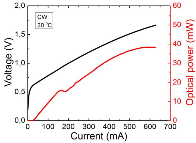
Fig. 2. Typical L-I-V characteristic
